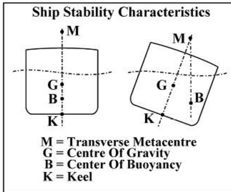
Figure 4. Basic Ship Stability Schematic
